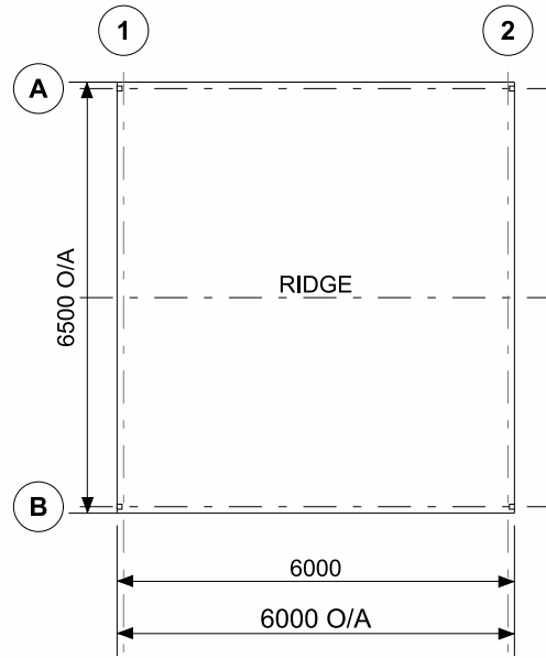
FRAME ROOF PLAN
