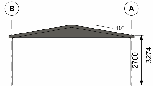
ELEVATION GRID 2
