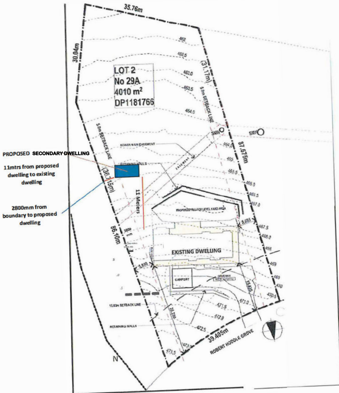
SITE PLAN – 29A ROBERT HODDLE ROAD MUDGEE
