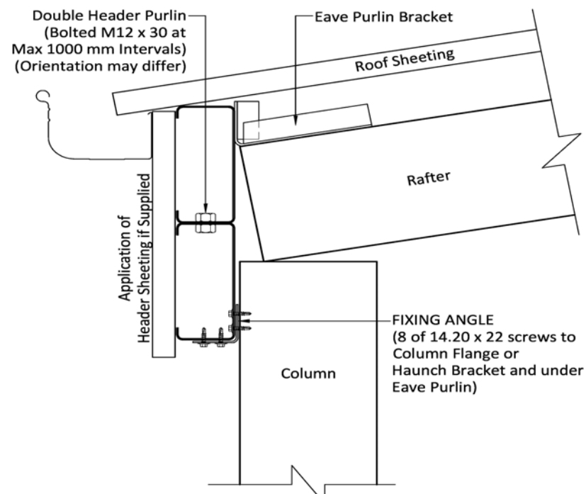
DOUBLE HEADER PURLIN CONNECTION - OPEN BAYS
