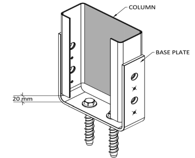
C150 COLUMN FIXING (BF) ○ FIXING BOLTS - 2 of M12 x 100 SCREWBOLT ○ FIXING BOLTS - 4 of M12 x 30 Galv. × FIXING SCREWS - 4 of 12.24 x 38 Series 500
