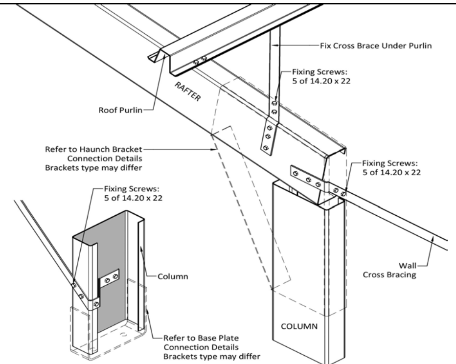
BRACING CONNECTION
