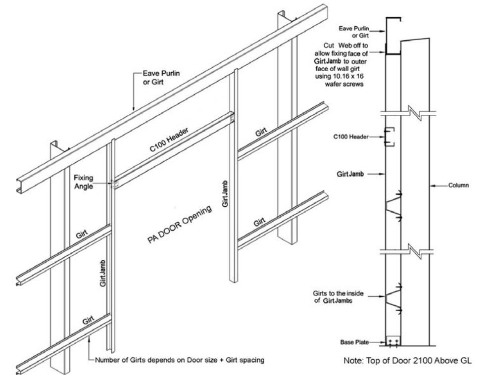
PA DOOR (PRE HUNG) CONNECTION DETAILS
