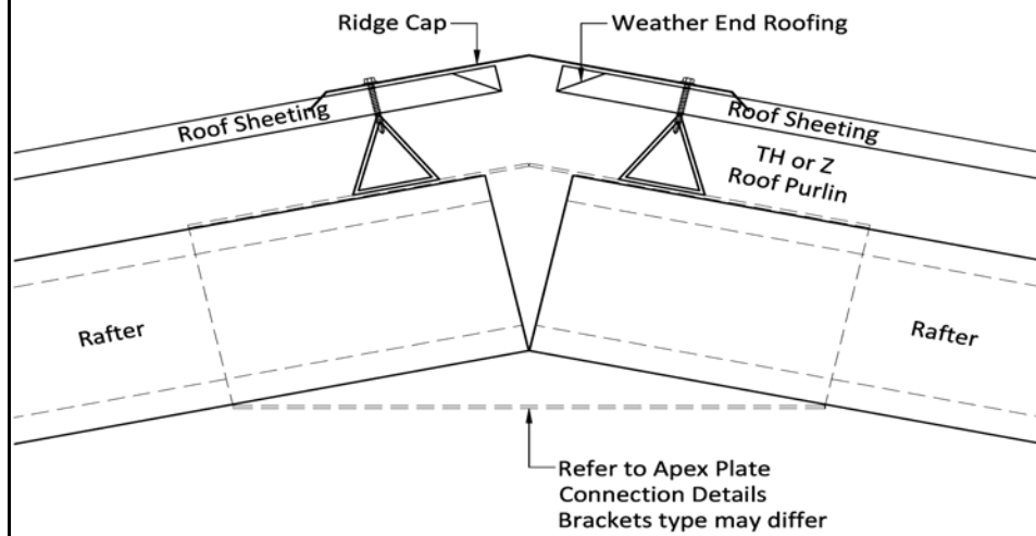
Ridge Cap - 2XF280
