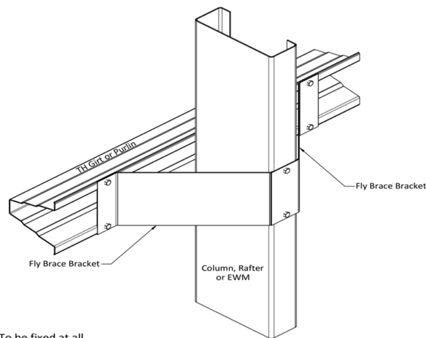
FLY BRACING BRACKET
